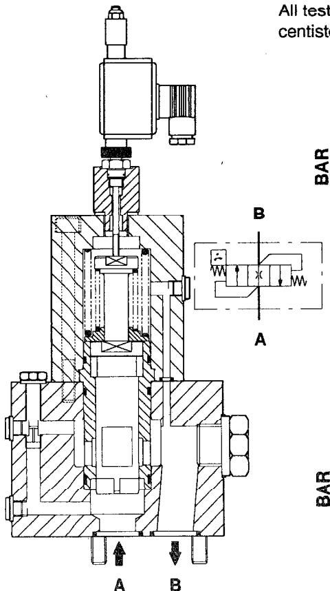
Flow switch. Switch operates with rising spool. Flow A to B.
