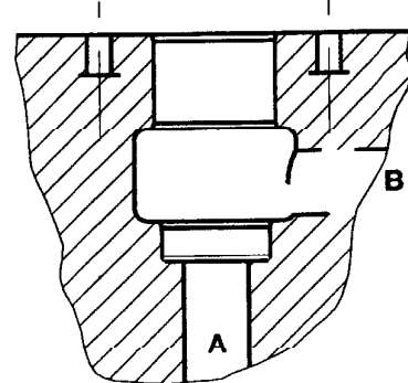
CAVITY FOR OVER 700 BAR
