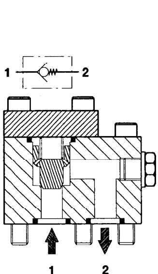
Traditional Range VCCS**E-A2S**N00KBA1
