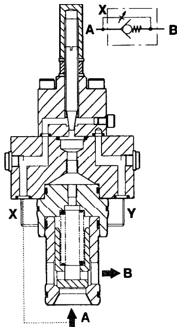
With adjustable bypass orifice VCCS**C-50S**B00MBA1
