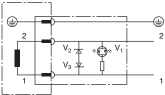
Connector wiring
