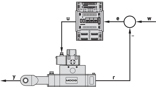
Control loop consisting of controller and valve-actuated cylinder with position transducer
