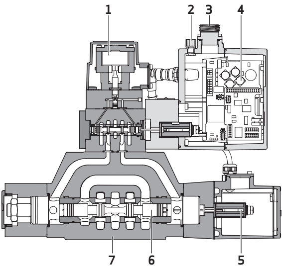
Cutaway view, 3-stage servovalve
