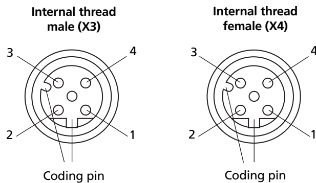
View on connection side of ETHERCAT receptacle
