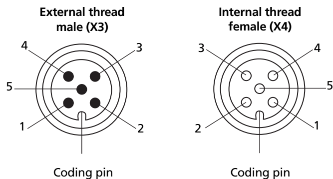
View on connection side of CANopen receptacle
