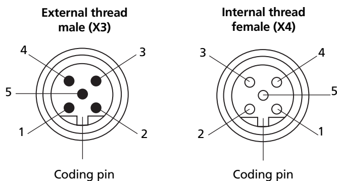
View on connection side of PROFIBUS-DP receptacle
