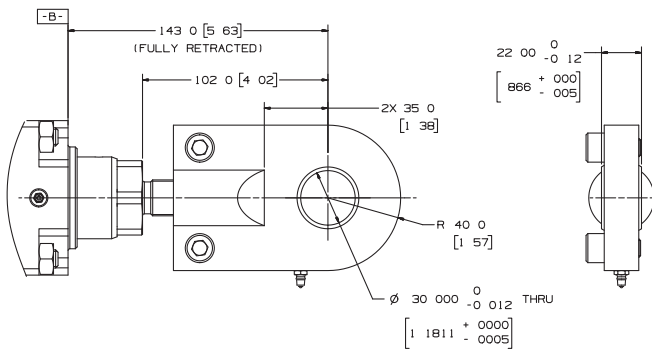
ROD END KIT, SPHERICAL BEARING OPTION (USED WITH INTERNAL ANTI-ROTATION) (CODE: 6)
