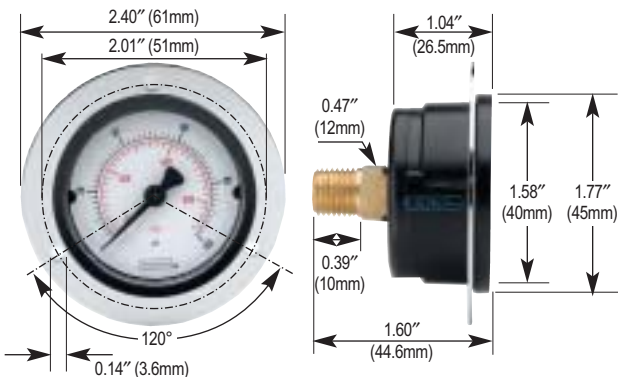
15-110 Front Flange
