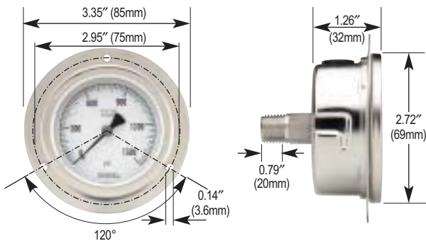
60-410/510 Front Flange
