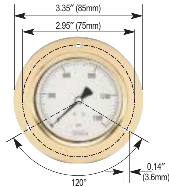
25-300 Rear Flange
