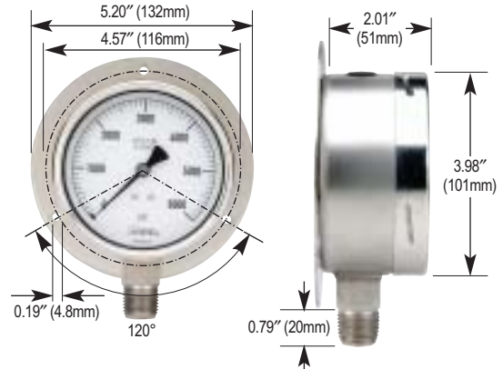
40-400/500 Rear Flange
