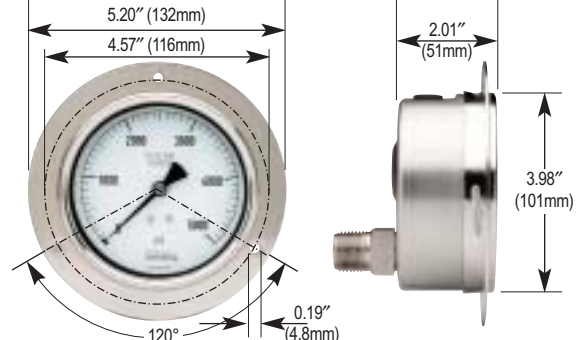
40-400/500 Rear Flange
