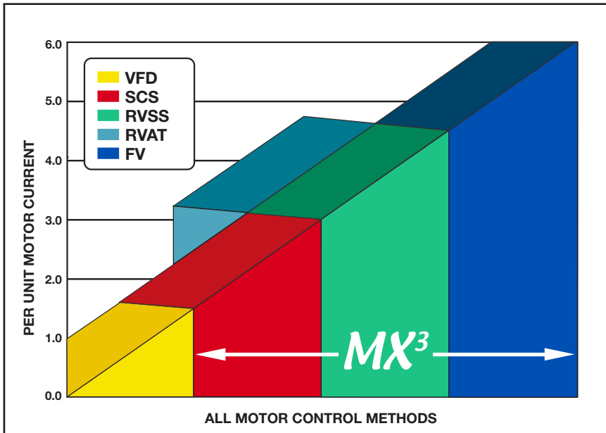
FIGURE 2. Starting current comparison.
