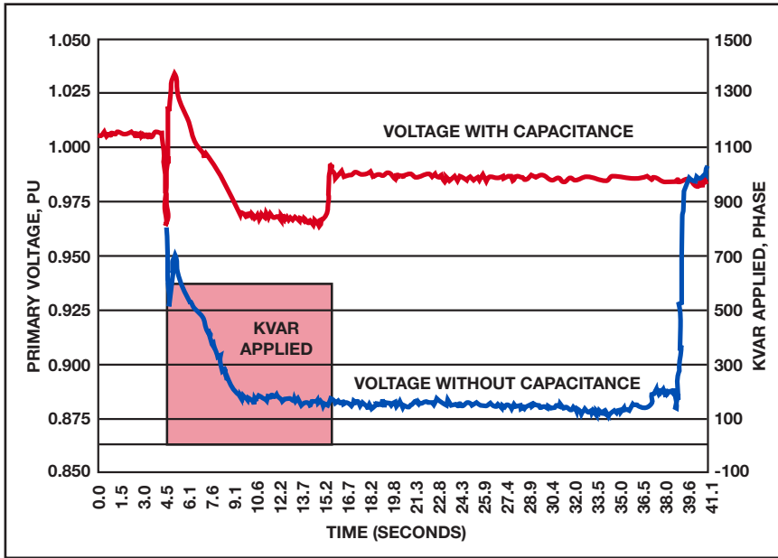
FIGURE 1. Motor start comparison with and without capacitance.
