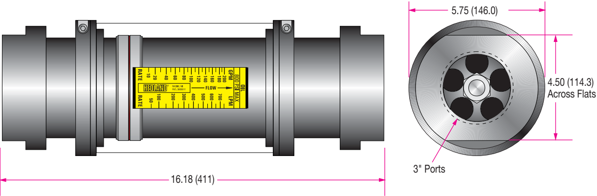
3 inch; SAE, NPTF, BSPP - Inches (mm)
