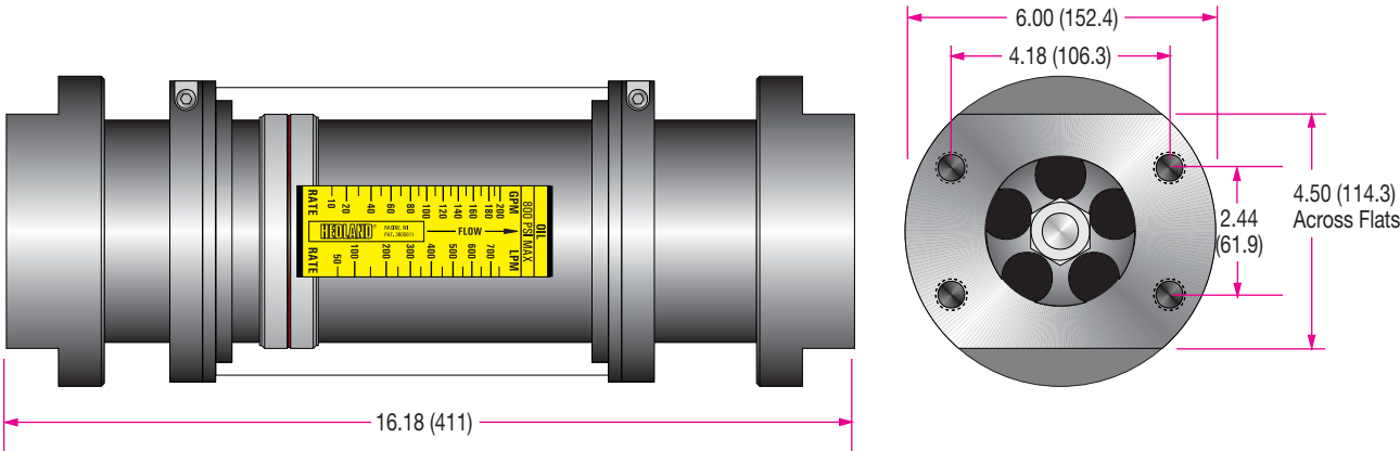
3 inch; C61 Flange - Inches (mm)
