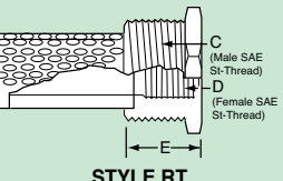
STYLE RT (Not stocked)
