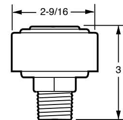
BF MODEL (3/4 NPT)
