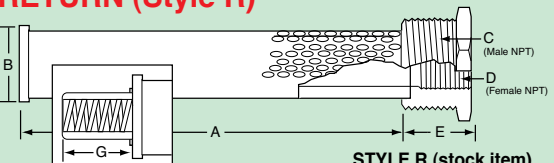
STYLE R (stock item) STYLE RFS (Not stocked)
